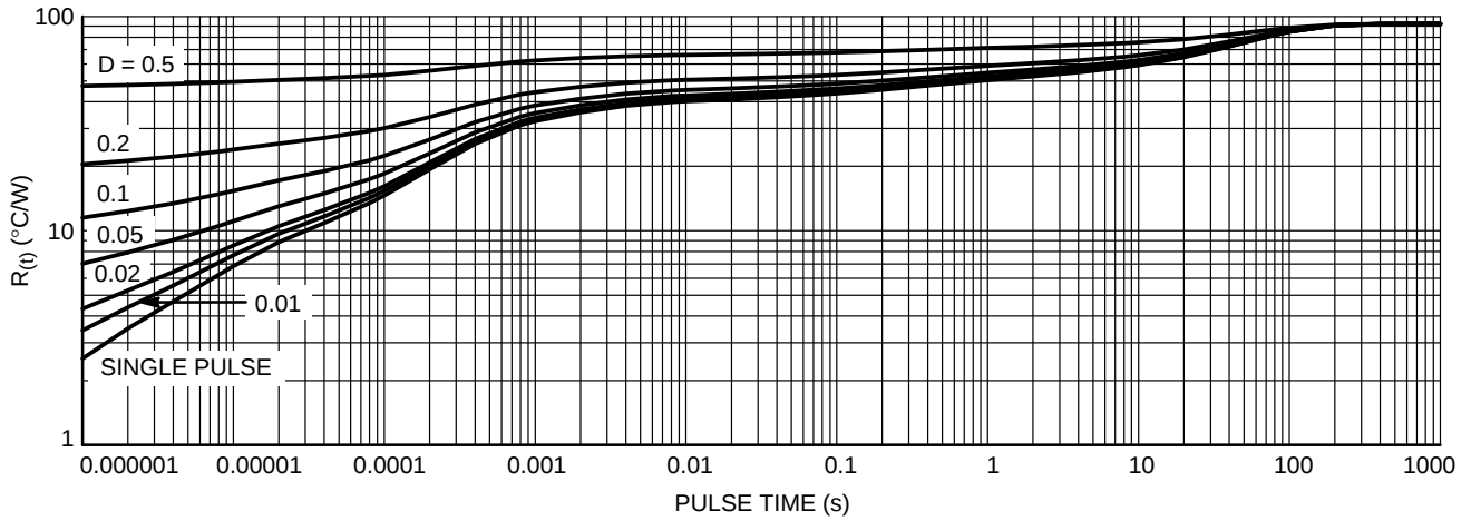
Figure 18. Thermal Duty Cycle Curves on 500 \text{ mm}^2 Spreader Test Board
