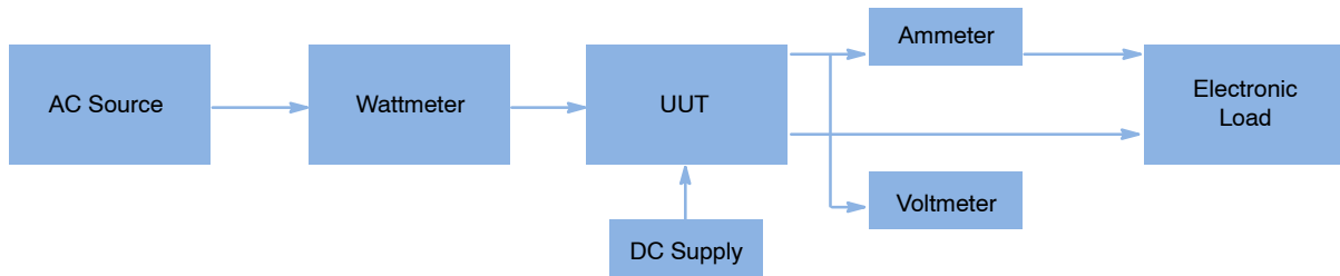
Figure 4. Test Setup
