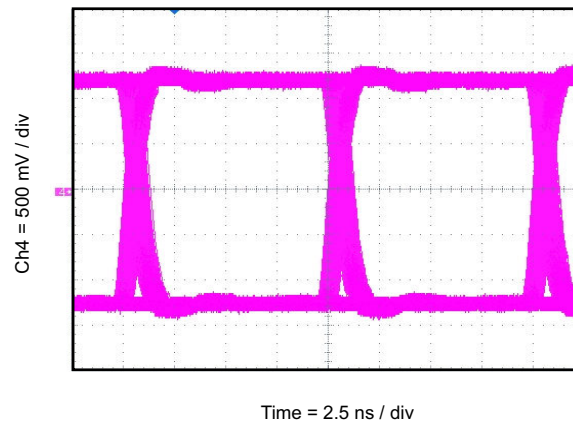
Figure 9-6. Eye Diagram at 100 Mbps PRBS 2^{16} - 1 , 2.5 V and 25°C
