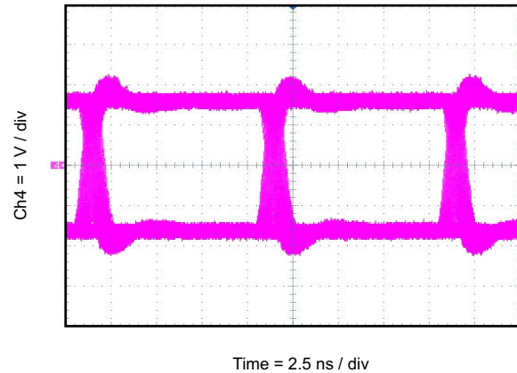
Figure 9-5. Eye Diagram at 100 Mbps PRBS 2^{16} - 1 , 3.3 V and 25°C
