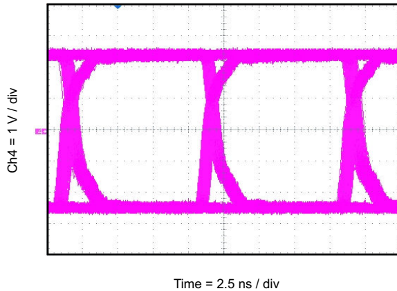
Figure 9-4. Eye Diagram at 100 Mbps PRBS 2^{16} - 1 , 5 V and 25°C
