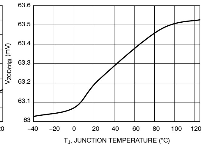
Figure 45. V ZCD(trig) vs. Temperature
