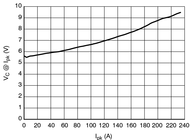
Figure 6. Clamping Voltage vs. Peak Pulse Current ( t_p = 8/20 \mu s ), Pin 2 to Pin 1
