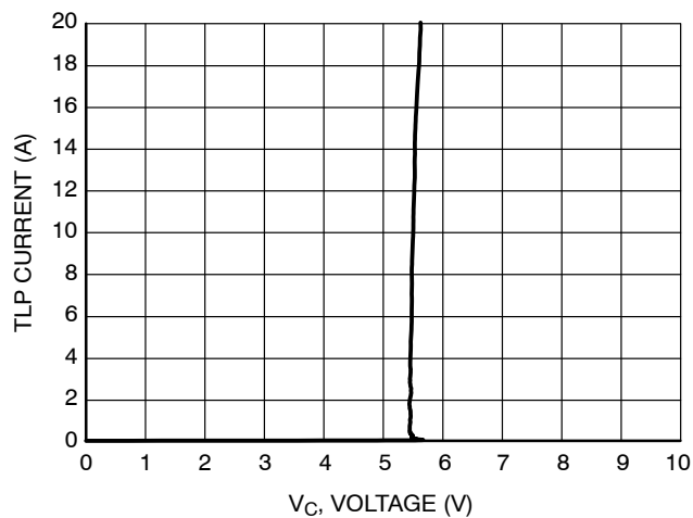
Figure 4. 100 ns TLP I-V Curve, Pin 2 to Pin 1
