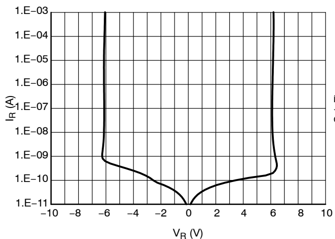
Figure 3. IV Characteristics
