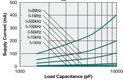
Supply Current vs. Load Capacitance ( V_{CC}=18V )
