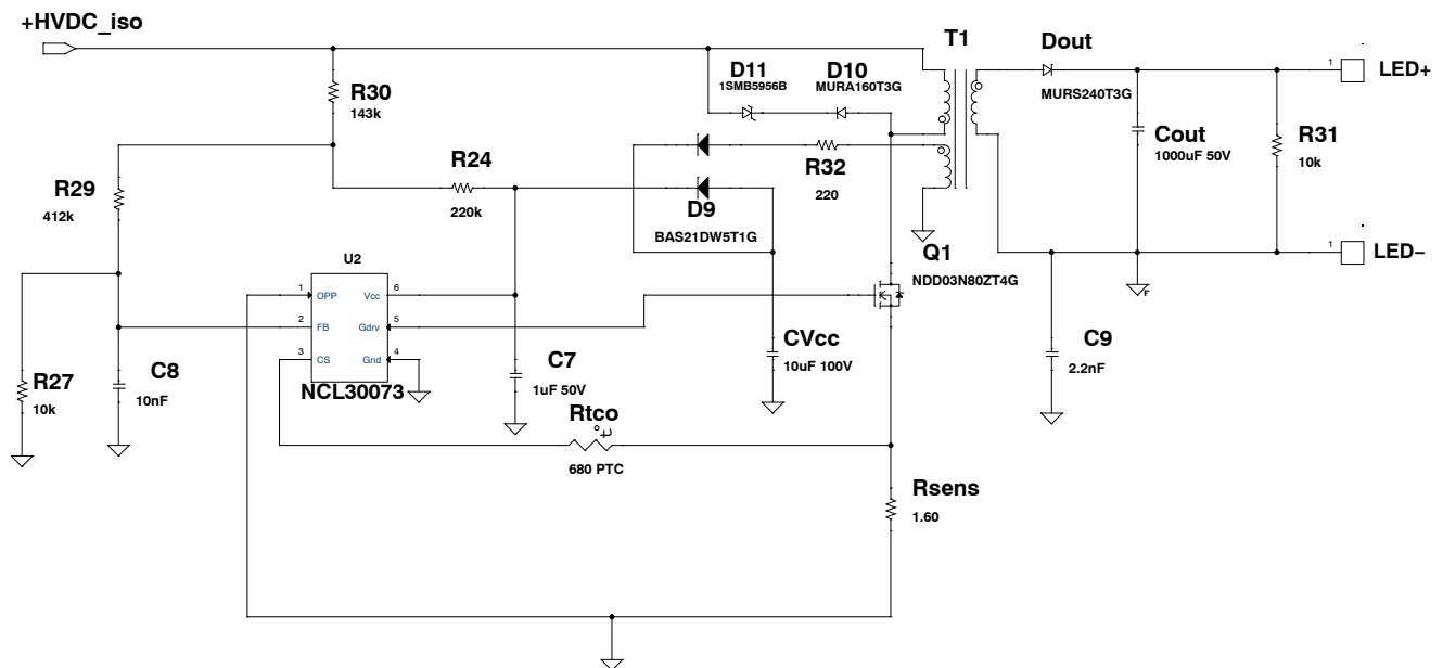
Figure 4. Main Circuit
