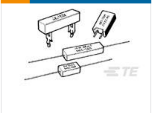
TE Part #1-1623789-8 SQM7 68R 5% (WIRE)
