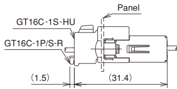
◆Mated condition
