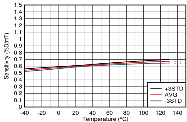
DRV5057A2, V_{CC} = 3.3 V
