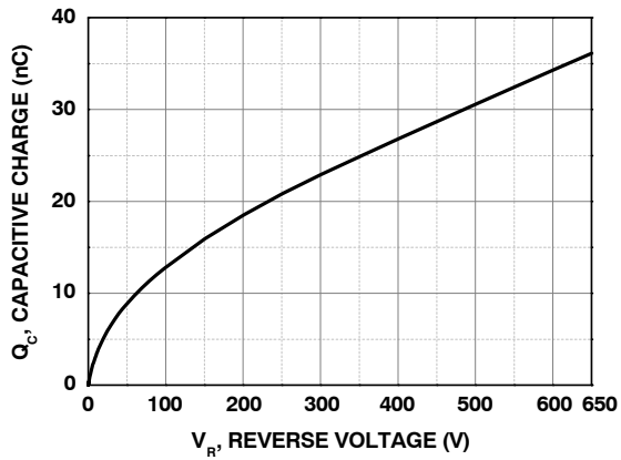
Figure 5. Capacitive Charge vs. Reverse Voltage
