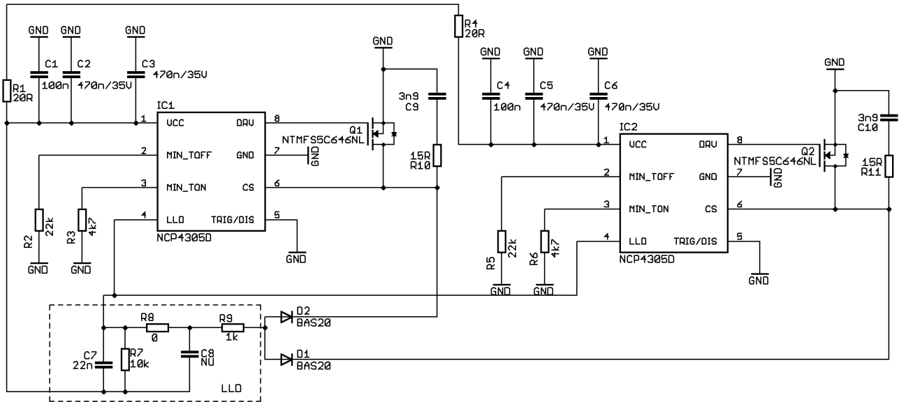
Figure 2. Laptop Adapter Demo-board – SR Daughtercard Schematic
