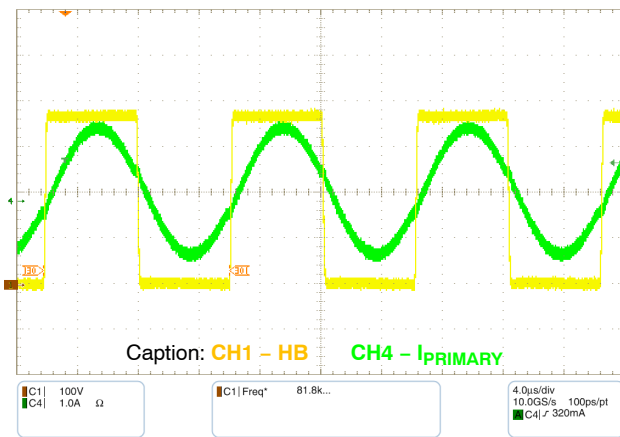
Figure 15. Steady Stage - I_{LOAD} = 8\text{ A}
