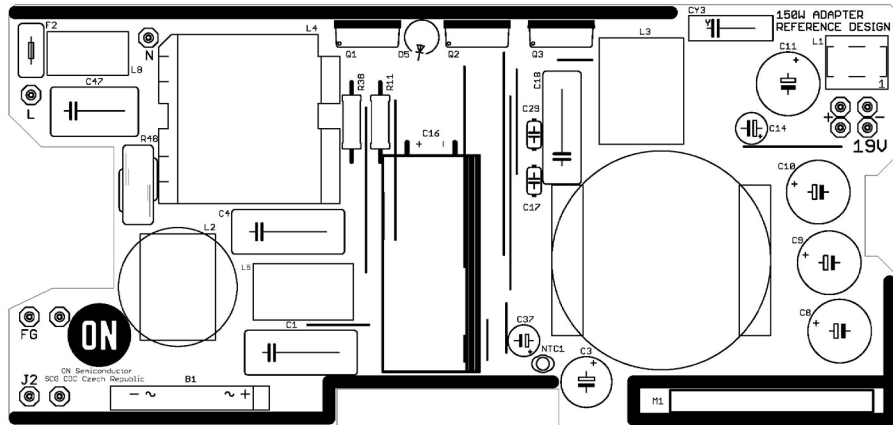
Figure 4. Main Board Top Side Components
