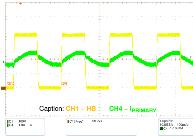
Figure 13. Steady Stage - I_{LOAD} = 2\text{ A}
