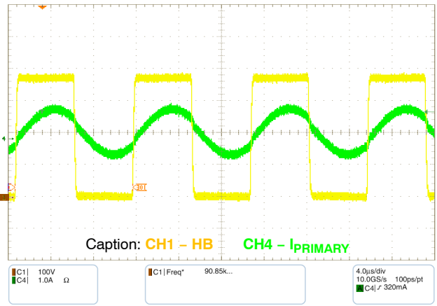
Figure 14. Steady Stage - I_{LOAD} = 4\text{ A}
