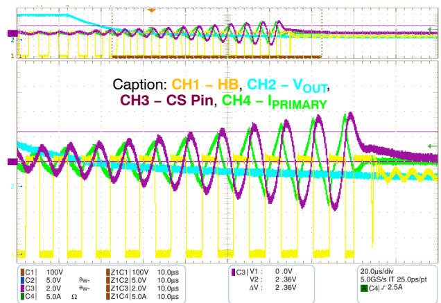
Figure 16. Secondary Short Transition
