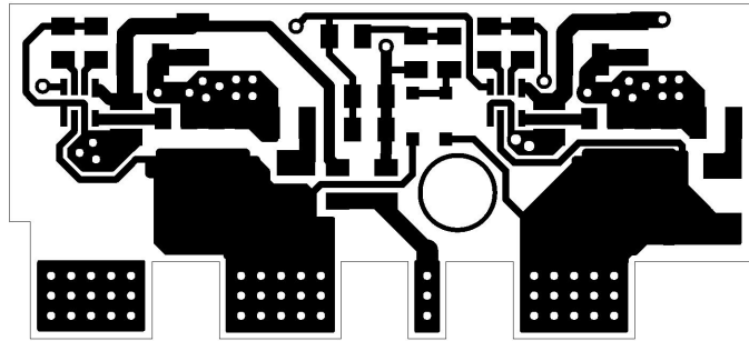
Figure 6. SR Daughtercard Board Top Layer
