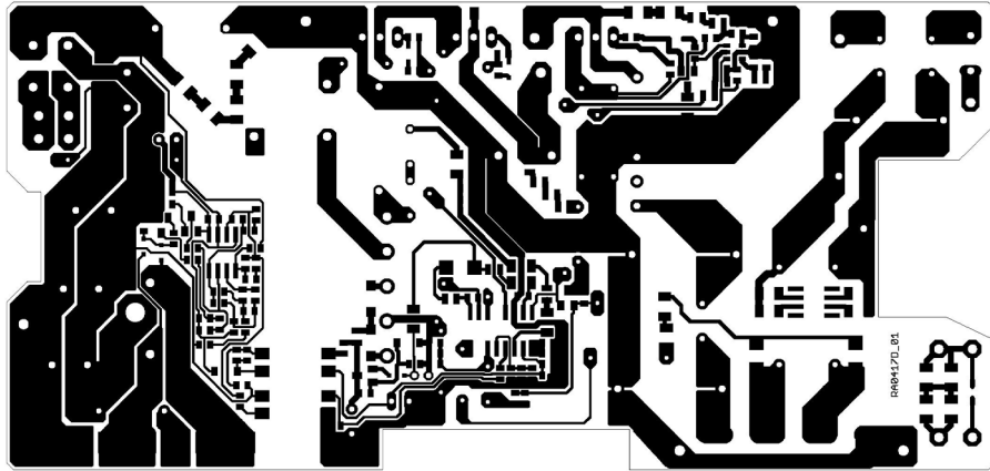
Figure 3. Main Board Bottom Layer
