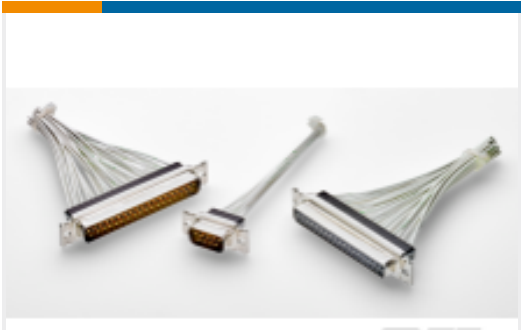
TE Part #2335891-2 AMPLIMITE SZ 2 PLUG 26 POS, ST STL SHEL
