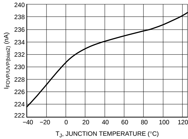
Figure 91. I FOVP/UVLP (bias2) vs. Temperature
