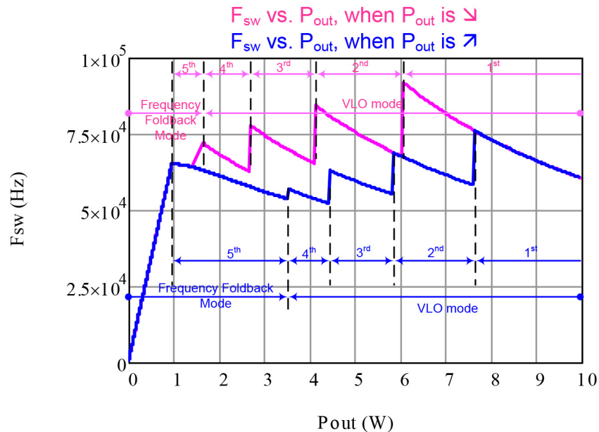
Figure 51. Typical Switching Frequency versus Output Power Relationship in a 10 W Adapter
