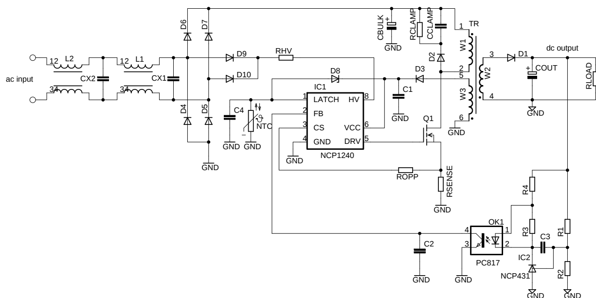
Figure 1. Flyback Converter Application Using the NCP1240G
