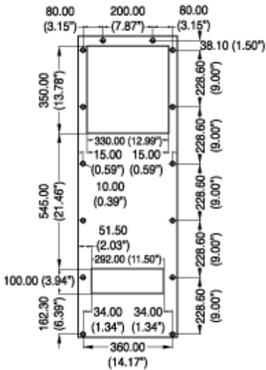
Drilling Template
