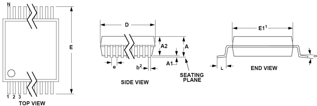
16L TSSOP (4.4 mm BODY) PACKAGE DRAWING
