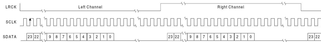
Figure 19. I 2 S Serial Audio Interface
