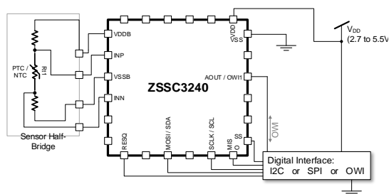
Sensor with Ratiometric Voltage Output and Digital Interface
