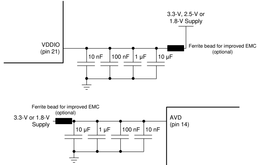
Figure 10-1. Power Connections
