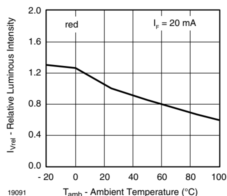
Fig. 30 - Relative Luminous Intensity vs. Ambient Temperature
