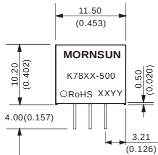
SIP-3 Package
