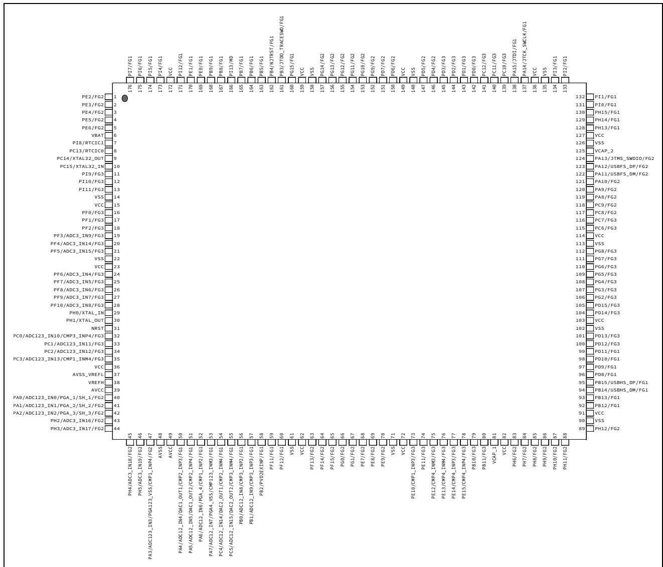
LQFP176
