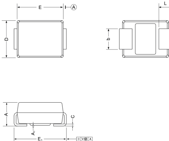
SMB mechanical data
