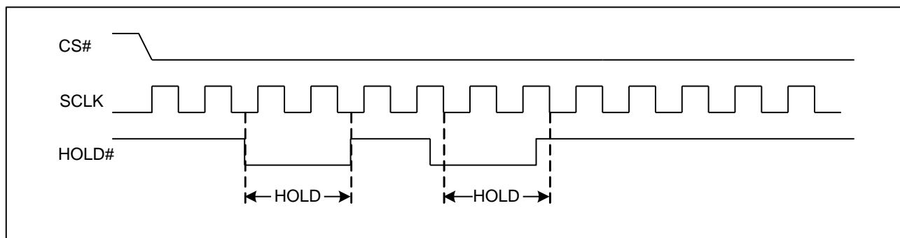
Figure 3 Hold Condition
