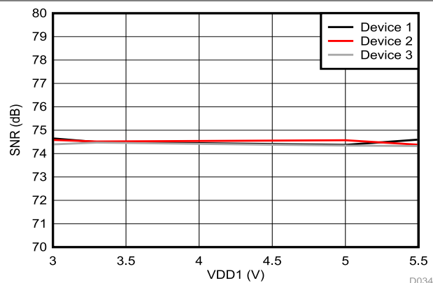
图 6-24. Signal-to-Noise Ratio vs High-Side Supply Voltage
