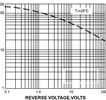
FIG. 5-TYPICAL JUNCTION CAPACITANCE
