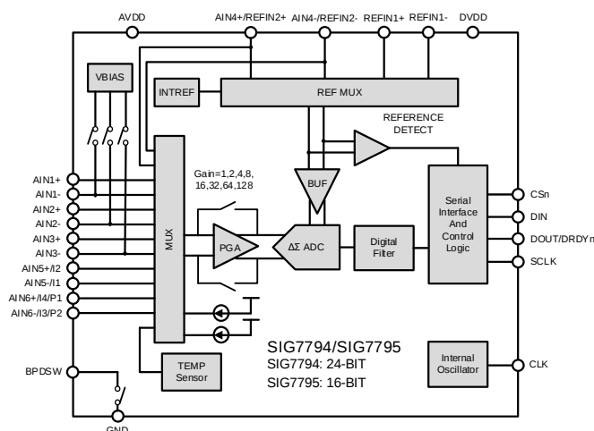
Function Block Diagram
