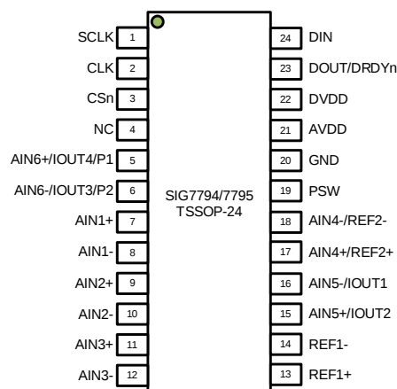
TSSOP-24
