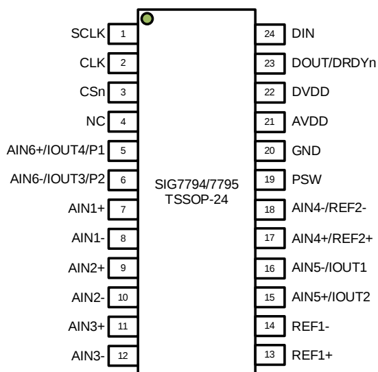
TOP VIEW (Not To Scale)
