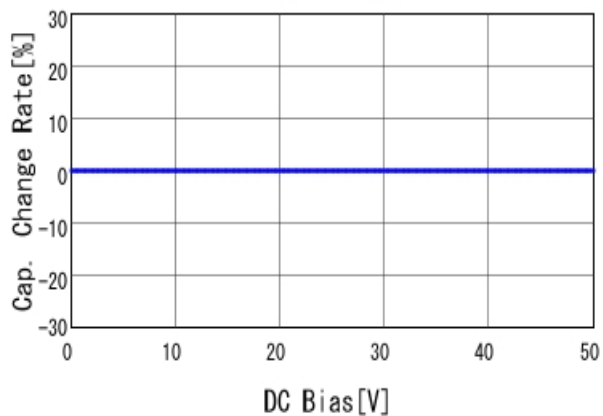
■ GRM1885C1HR80WA01 C-DC bias capchange, 25.0degC, AC1V
