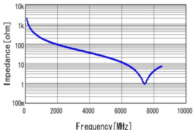
■ GRM1885C1HR80WA01 |Z| DCOV, 25degC
