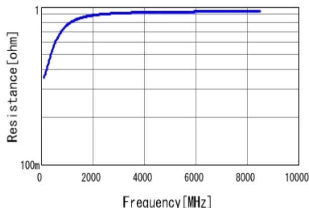
■ GRM1885C1HR80WA01 R DCOV, 25degC
