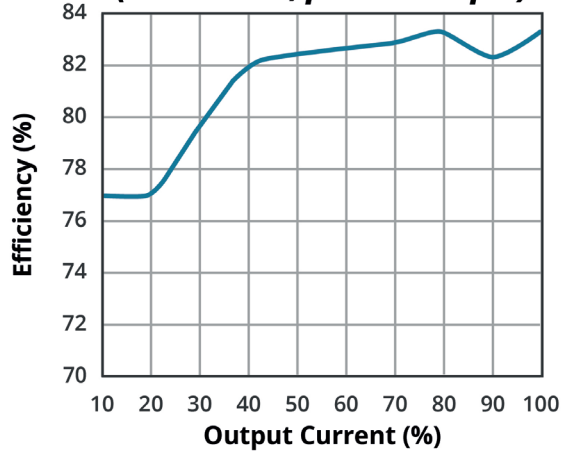
EFFICIENCY VS OUTPUT LOAD VX78012-500 (nominal Vin, positive output)
