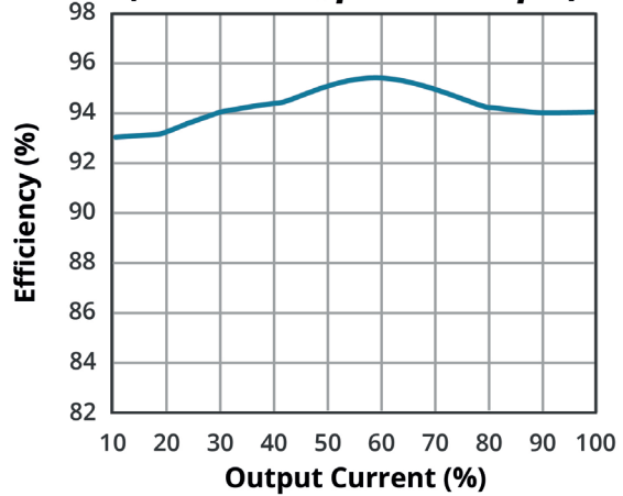
EFFICIENCY VS OUTPUT LOAD VX78012-500 (nominal Vin, positive output)
