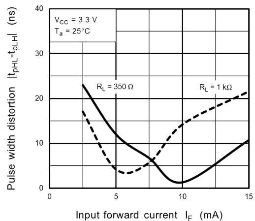
Fig. 12.2.22 |t_{pHL} - t_{pLH}| - I_F
