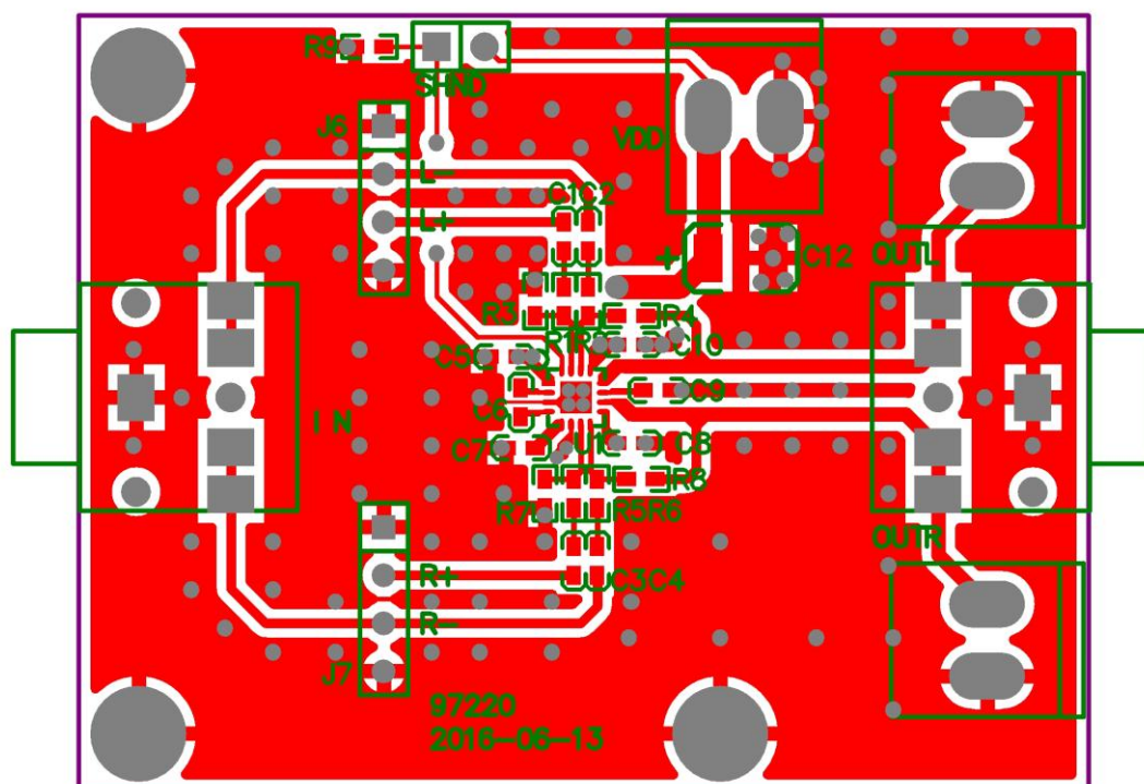
Fig.4 Top View of HT97220L/HT4917 Demo Board PCB Layout
