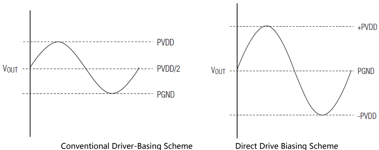
Fig. 1 Conventional Driver Output Waveform vs. HT97220L/HT4917 Output Waveform
