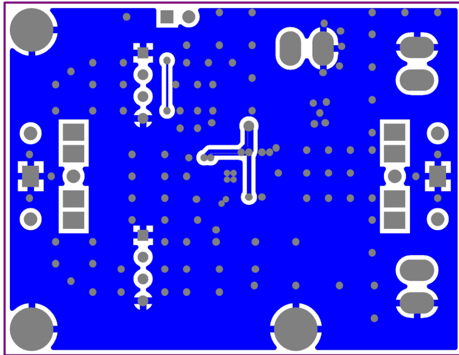
Fig.5 Bottom View of HT97220L/HT4917 Demo Board PCB Layout
