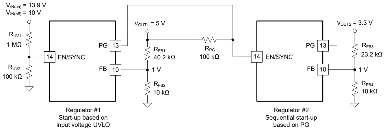
图 8-3. TPSM63604 Sequencing Implementation Using PG and EN/SYNC
