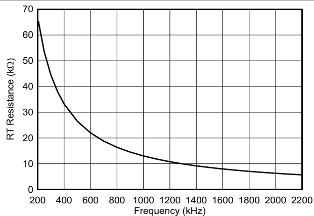
图 7-8. Switching Frequency Set by RT Resistor
