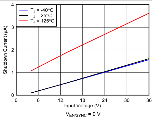
图 7-1. Shutdown Supply Current
