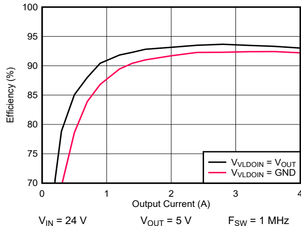
图 8-5. Efficiency Increase With External Bias
