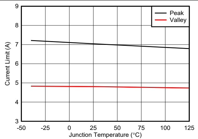
图 7-4. High-Side (Peak) and Low-Side (Valley) Current Limits
