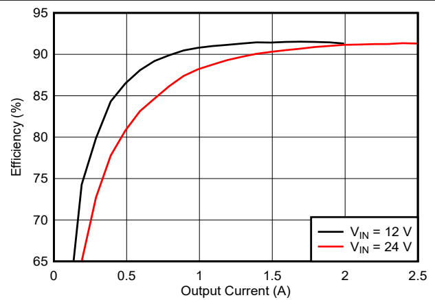
图 9-12. Efficiency
