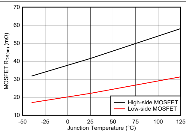
图 7-5. High-Side and Low-Side MOSFET R_{DS(on)}
