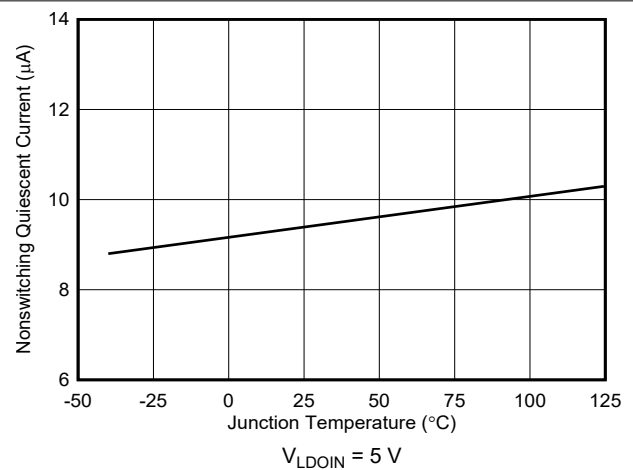
图 7-2. Nonswitching Input Supply Current
