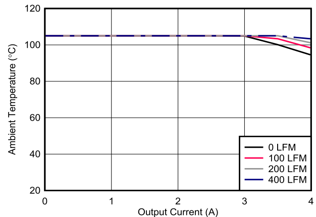
图 7-17. Safe Operating Area ( V_{OUT} = 3.3\text{ V} , F_{SW} = 750\text{ kHz} )
