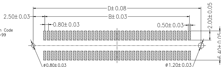
Recommended P.C.B Layout(Top Side)
