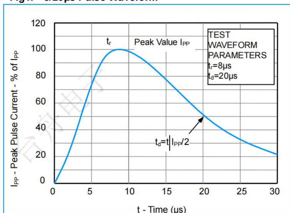
Fig1. 8/20 \mu s Pulse Waveform
