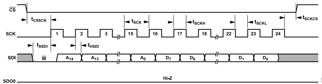
Figure 3. Register Configuration Mode Write Timing
