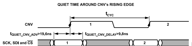
Figure 57. Quiet Zones
