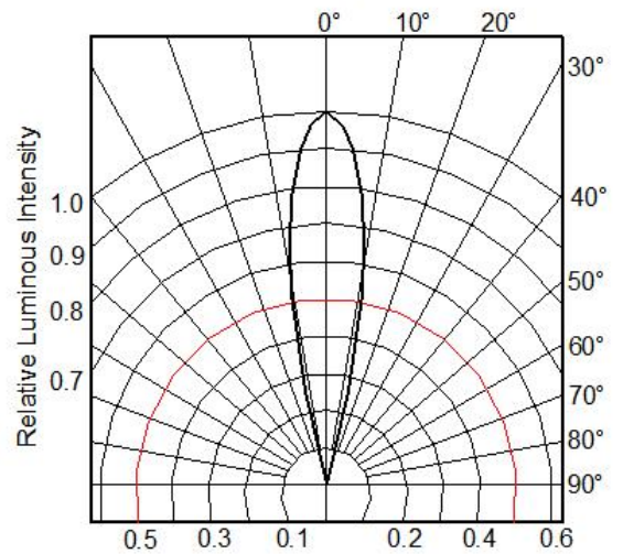
Fig.6 Radiation diagram(Ta=25°C)
