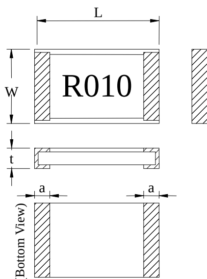
Figure 1. Construction Dimensions
