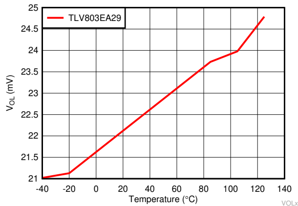
图 7-13. Low Voltage Output Versus Temperature for TLV803EA29, V_{DD} = 1.7\text{ V}
