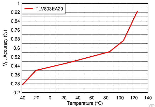
图 7-9. Voltage Threshold Accuracy Versus Temperature for TLV803EA29
