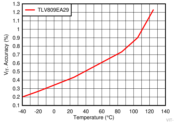
图 7-10. Voltage Threshold Accuracy Versus Temperature for TLV809EA29
