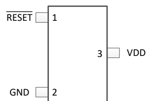
图 6-3. DBZ Package (Pin 1 = RESET, R pinout) 3-Pin SOT-23 Top View
