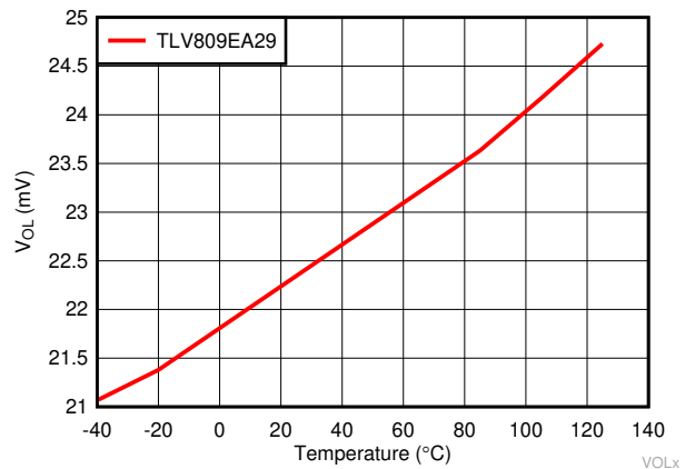
图 7-14. Low Voltage Output Versus Temperature for TLV809EA29, V_{DD} = 1.7\text{ V}
