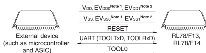
Figure 30-3. Environment for Writing Program to Flash Memory
