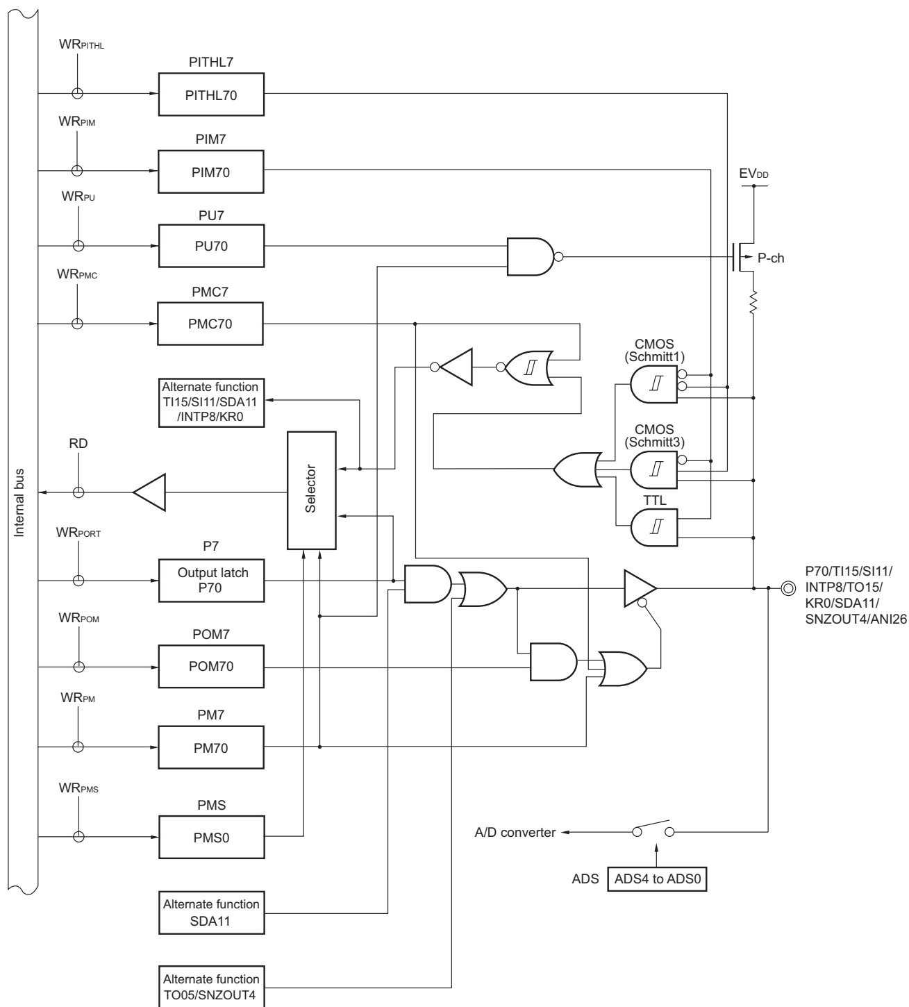
Figure 4-41. Block Diagram of P70
