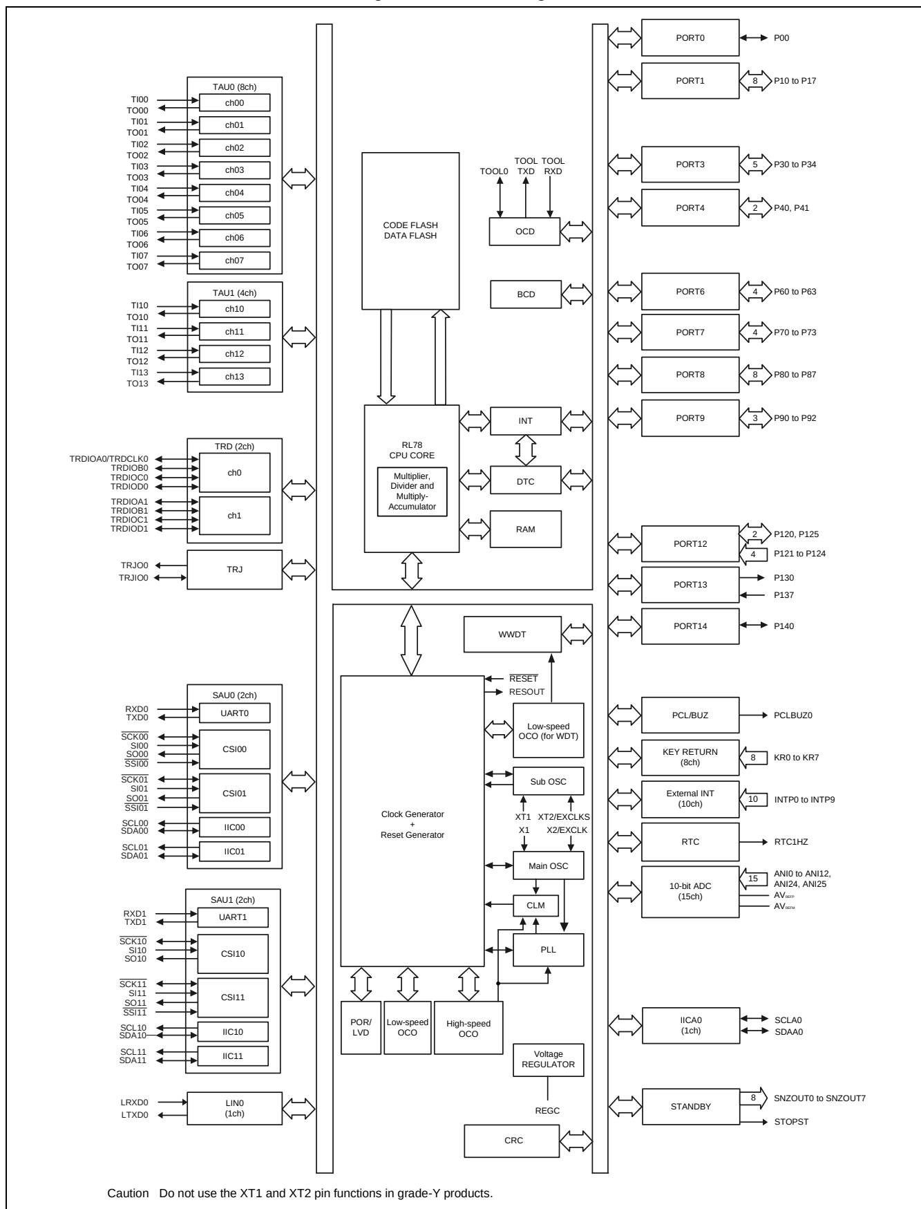
Figure 1-17. Block Diagram
