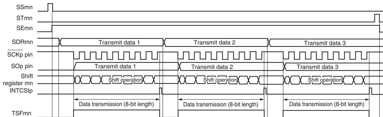
Figure 15-53. Timing Chart of Slave Transmission (in Single-Transmission Mode)
