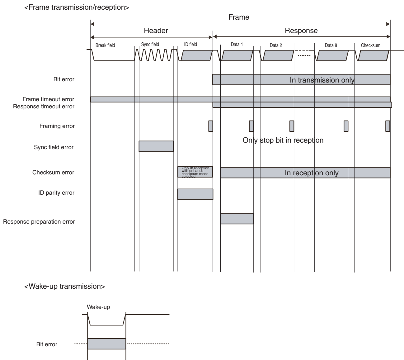
Figure 17-21. Target Time Area for LIN Error Detection (LIN Slave Mode)
