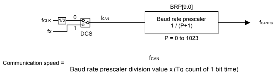
Figure 18-18. CAN Clock Control Block Diagram
