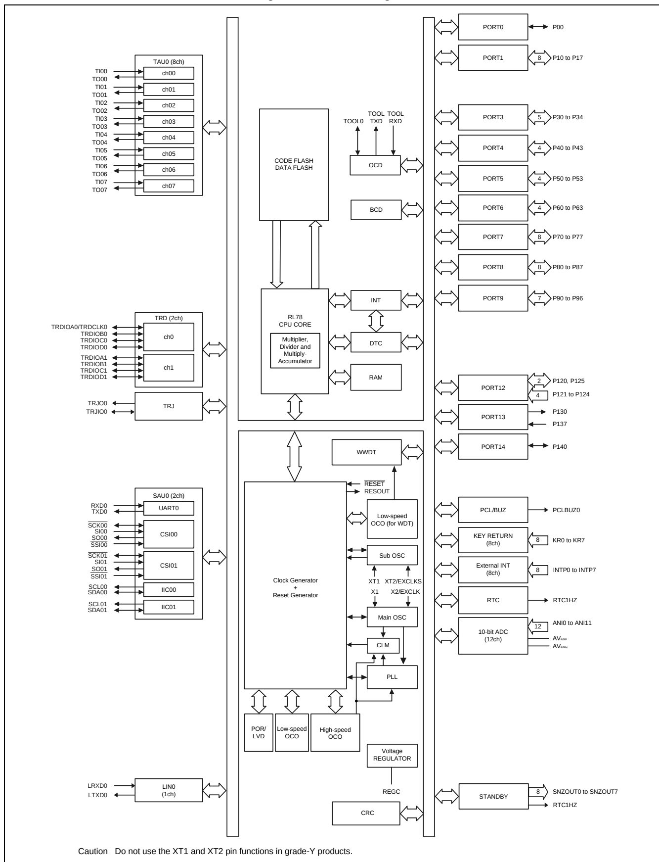
<R> Figure 1-18. Block Diagram
