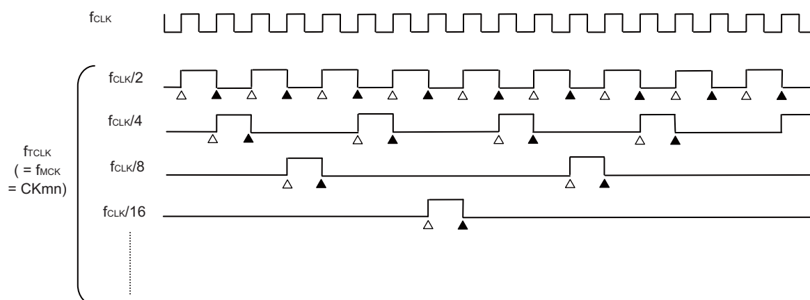
Figure 6-27. Timing of f_{\text{CLK}} and count clock ( f_{\text{TCLK}} ) (When CCSmn = 0)
