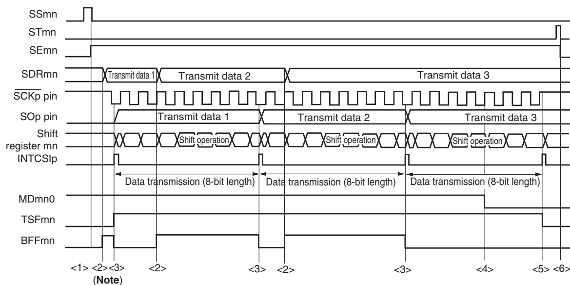
Figure 15-55. Timing Chart of Slave Transmission (in Continuous Transmission Mode)
