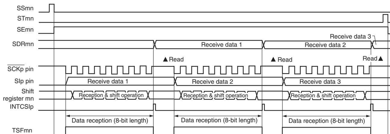
Figure 15-61. Timing Chart of Slave Reception (in Single-Reception Mode)
