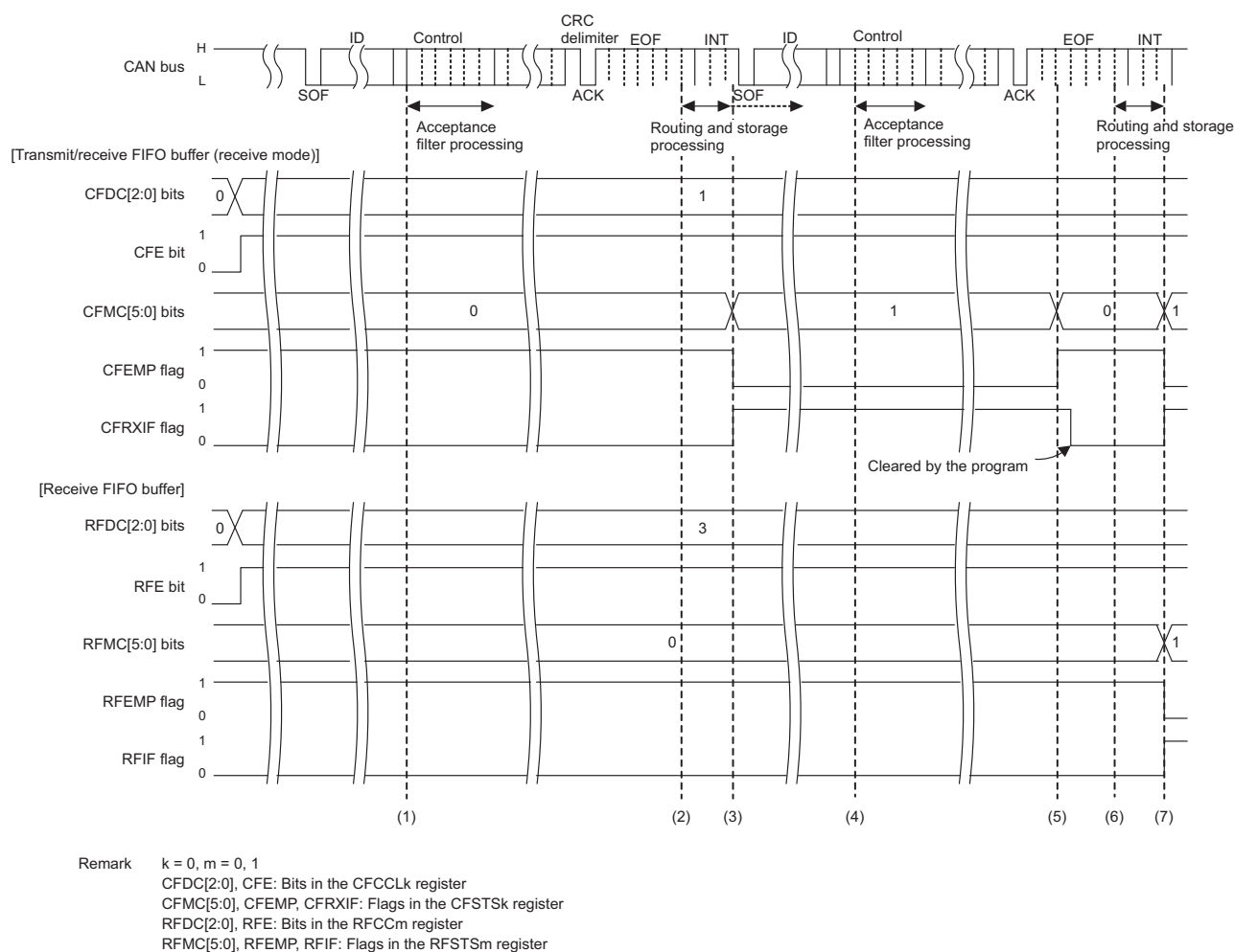
Figure 18-25. FIFO Buffer Reception Timing Chart
