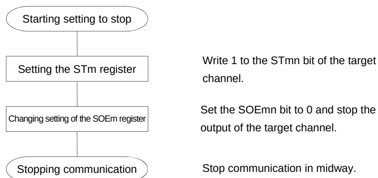
Figure 15-114. Procedure for Stopping Slave Transmission/Reception
