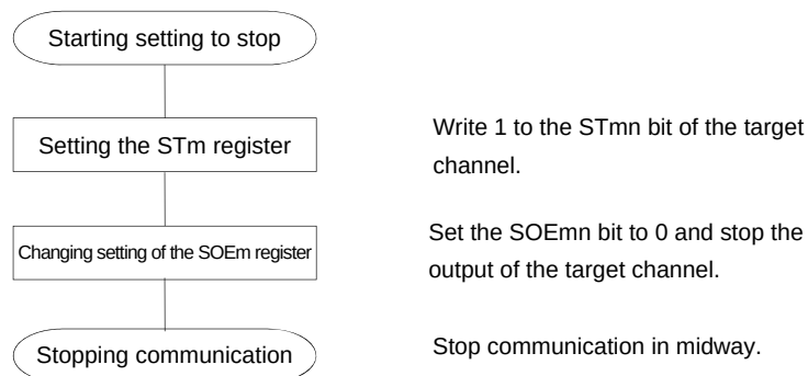
Figure 15-92. Procedure for Stopping Master Transmission/Reception
