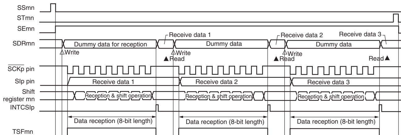
Figure 15-37. Timing Chart of Master Reception (in Single-Reception Mode)
