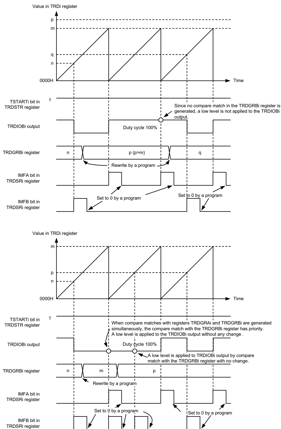
Figure 8-54. Operation Example in PWM Function (Duty Cycle 0%, Duty Cycle 100%)
