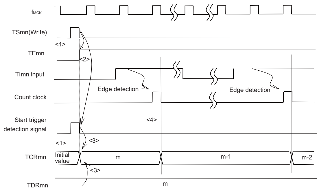
Figure 6-30. Start Timing (In Event Counter Mode)
