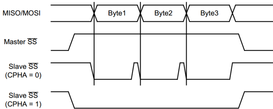
Figure 14-5 CPHA/SS 时序
