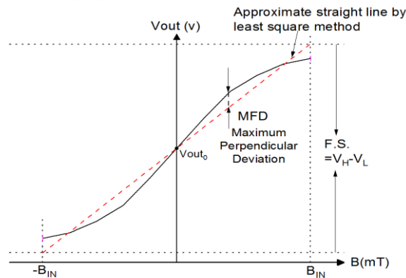
Figure 1. Output characteristics of GS302SA
