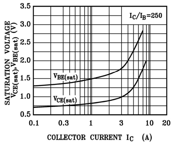
Fig 2. V_{CE(sat)} , V_{BE(sat)} vs. Collector Current
