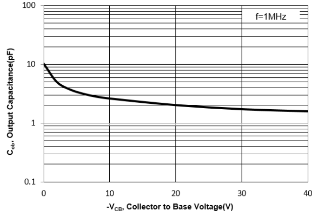
Fig 6. Capacitance Characteristics
