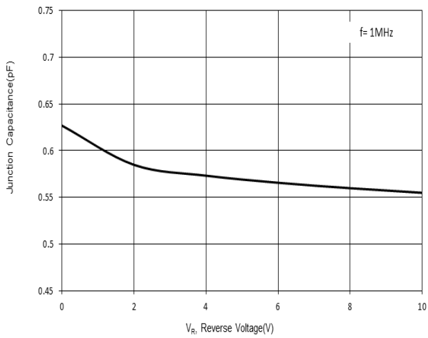
Fig 3. Junction Capacitance
