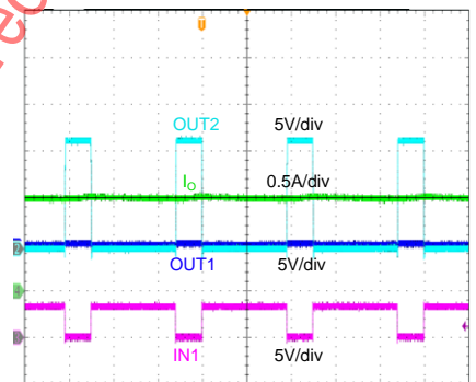
Operation Waveform (VM=12V, Io=1A, IN1=PWM, IN2=High)
