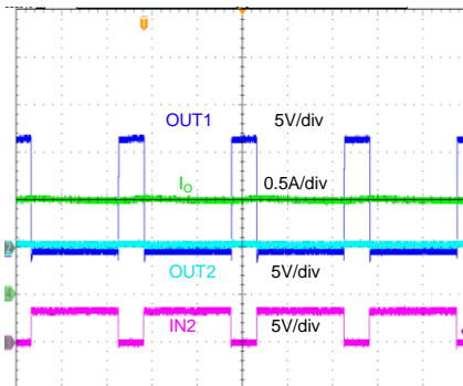
Operation Waveform (VM=12V, Io=1A, IN2=PWM, IN1=High)
