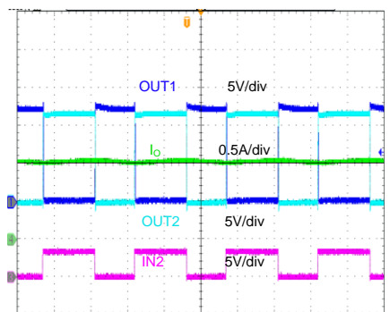
Operation Waveform (VM=12V, Io=1A, IN2=IN1)
