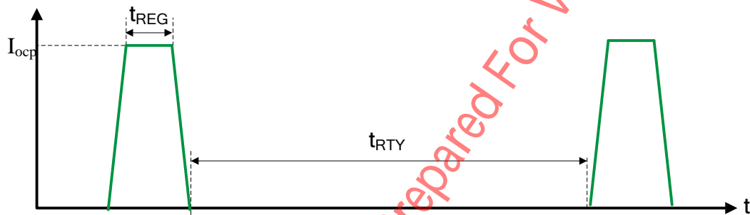
Figure 4. OCP schematic
