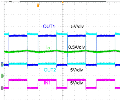
Operation Waveform (VM=12V, Io=1A, IN1=PWM)
