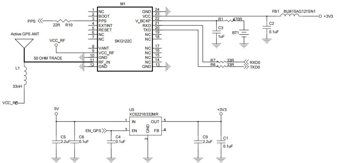
SKG122C 参考电路/ SKG122C Reference Circuit
