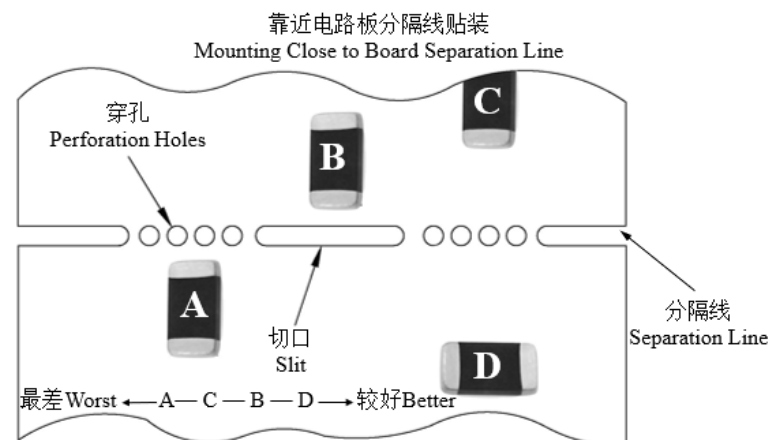
使本产品放在印刷电路板上靠近切口, 而不是靠近穿孔。 Put this product on the PC Board near the Slit, not near the Perforation Holes.
