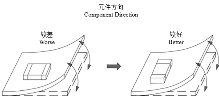
将产品沿应力作用方向水平放置。 Locate this product horizontal to the direction in which stress acts.
