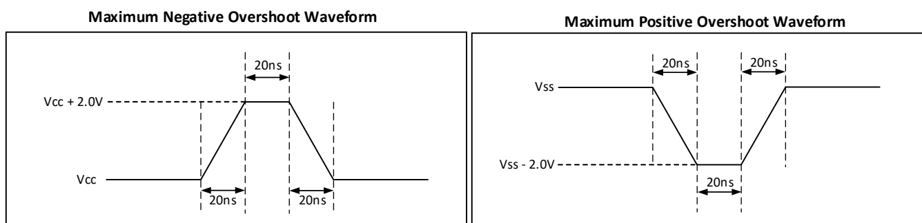
Figure-30. Maximum Negative/positive Overshoot Diagram
