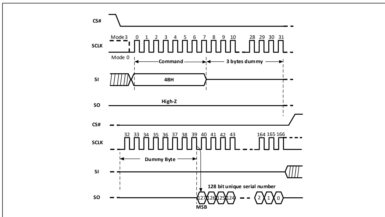
Figure-28. Read Unique ID Sequence Diagram
